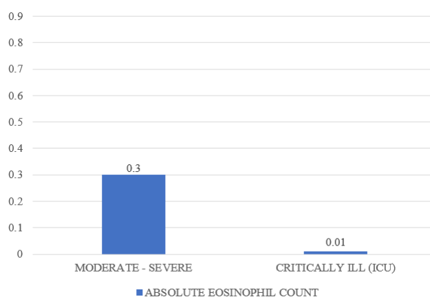
Fig. 1: Comparison of Absolute eosinophil count between Moderate to severe cases and critically ill patients
